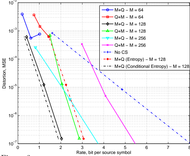
Figure 3: Rate Distortion performance, Q+M vs. M+Q systems. N = 512 , K_C = K_j = 8 , \alpha = 10^{-2}
