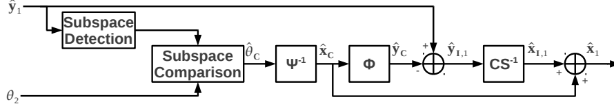
Figure 2: Block diagram of the Joint Reconstruction stage
