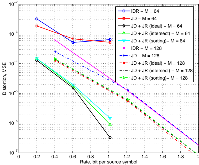
Figure 4: Rate-distortion performance, Joint dequantization and Joint reconstruction. N = 512 , K_C = K_j = 8 , \alpha = 10^{-2}
