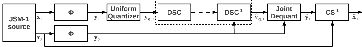
(a) Block diagram of the Measure-then-quantize system
