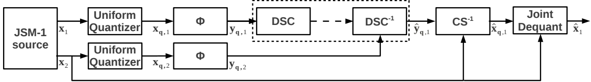
(b) Block diagram of the Quantize-then-measure system
